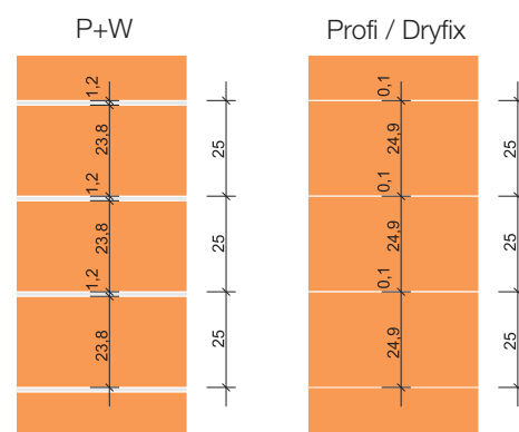
Porotherm P+W / Profi / Dryfix
