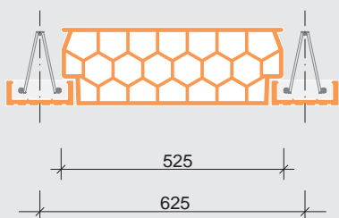
Strop Porotherm 62.5
