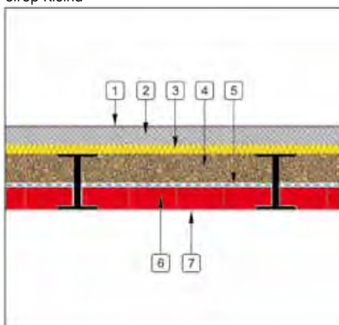
Strop Kleina
